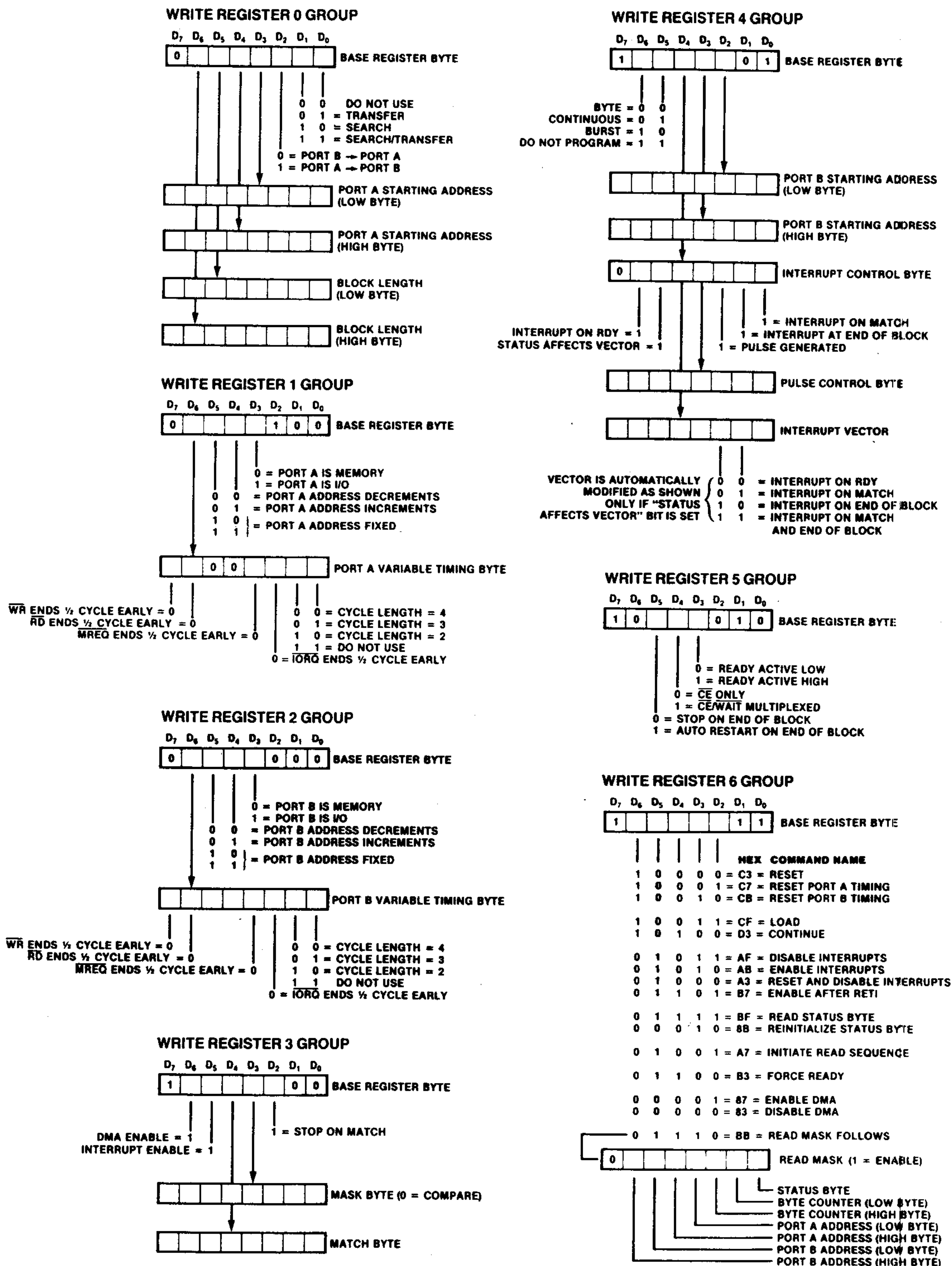
Figure 8b. Write Registers
