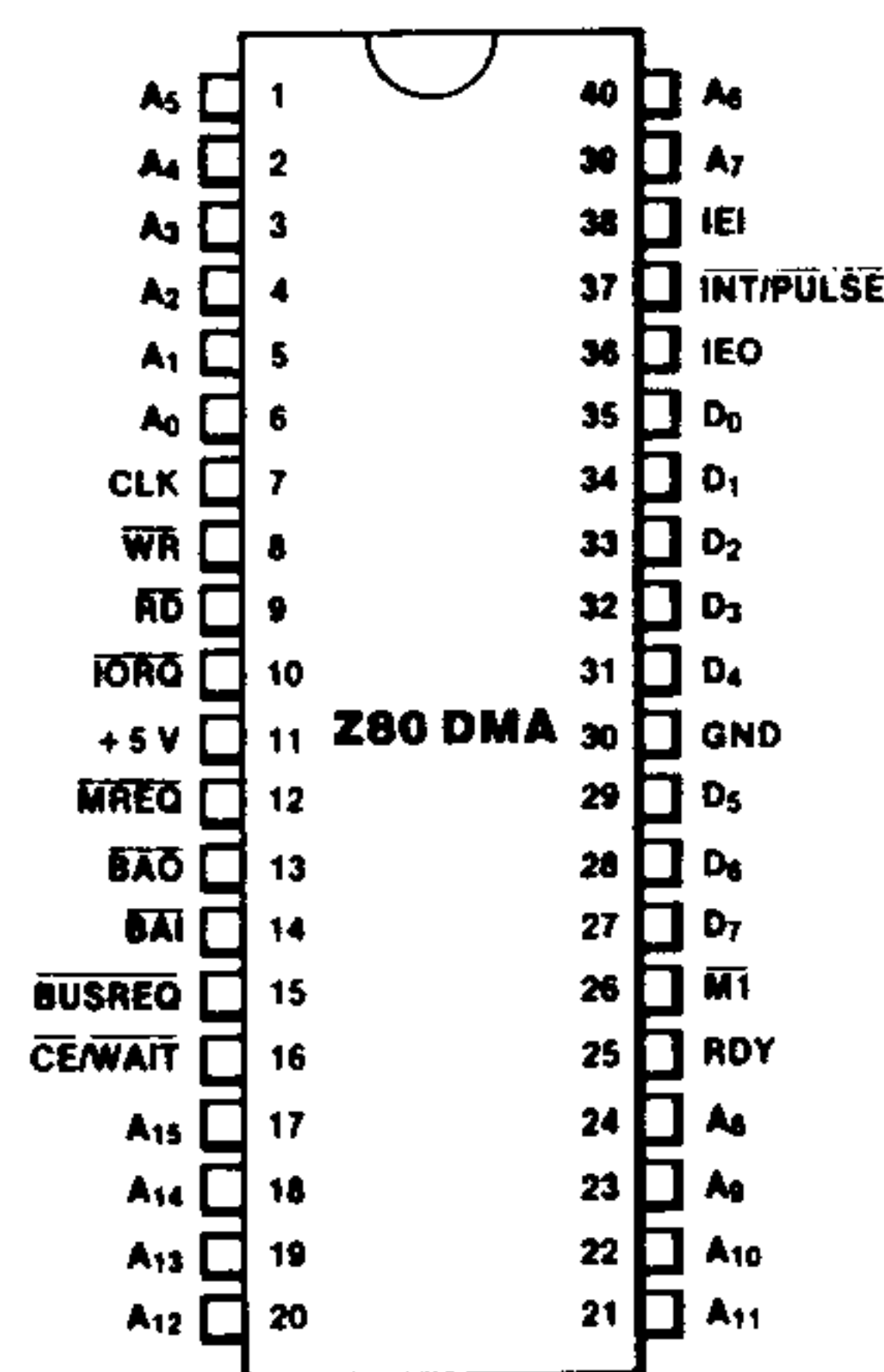
Figure 2a. 40-pin Dual-In-Line Package (DIP), Pin Assignments
