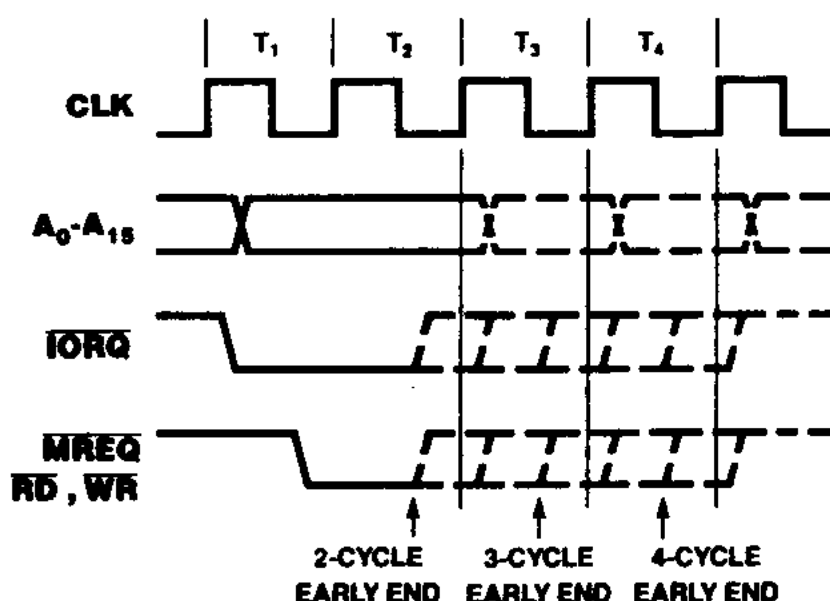
Figure 14. Variable-Cycle and Edge Timing
