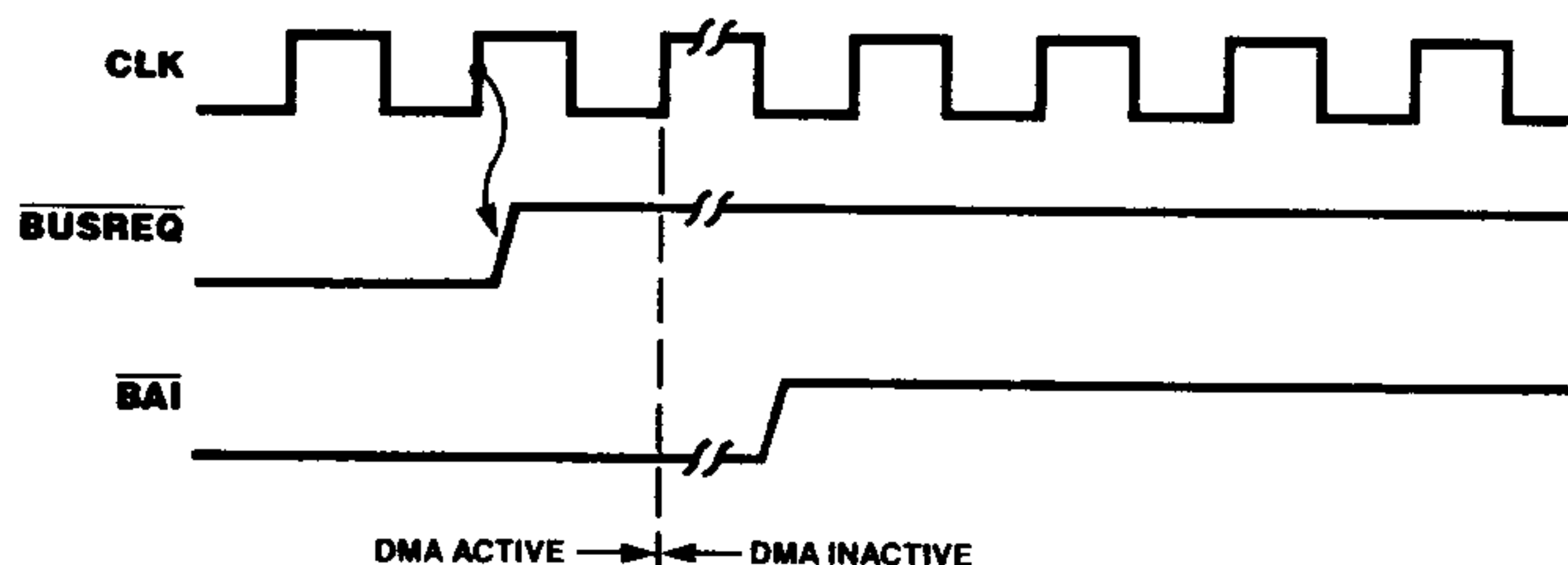
Figure 16. Bus Release (Byte-at-a-Time Mode)
