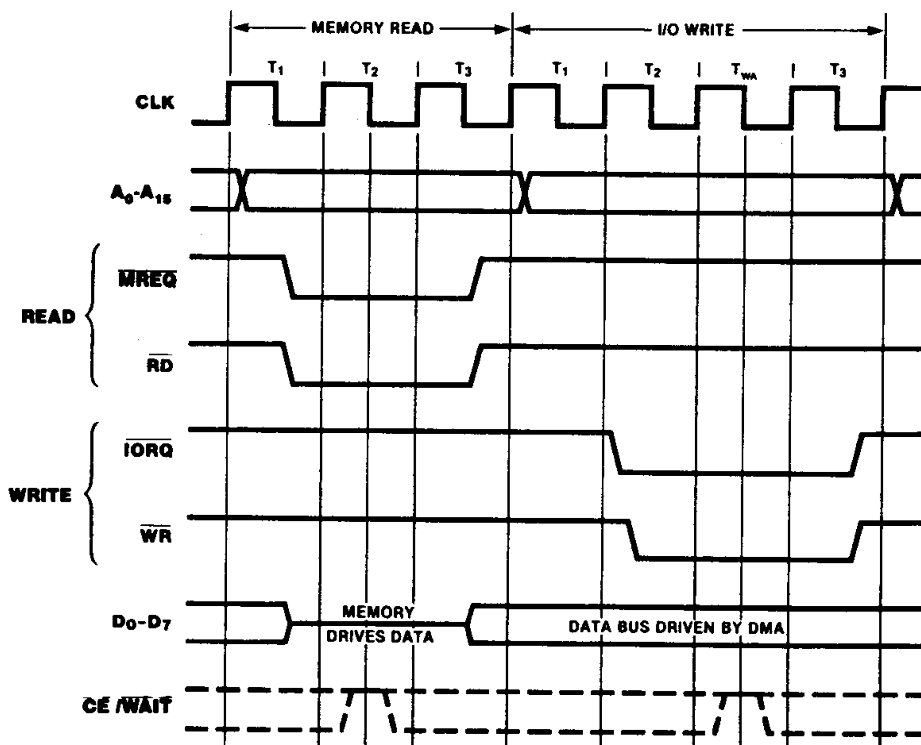
Figure 12. Memory-to-I/O Transfer
