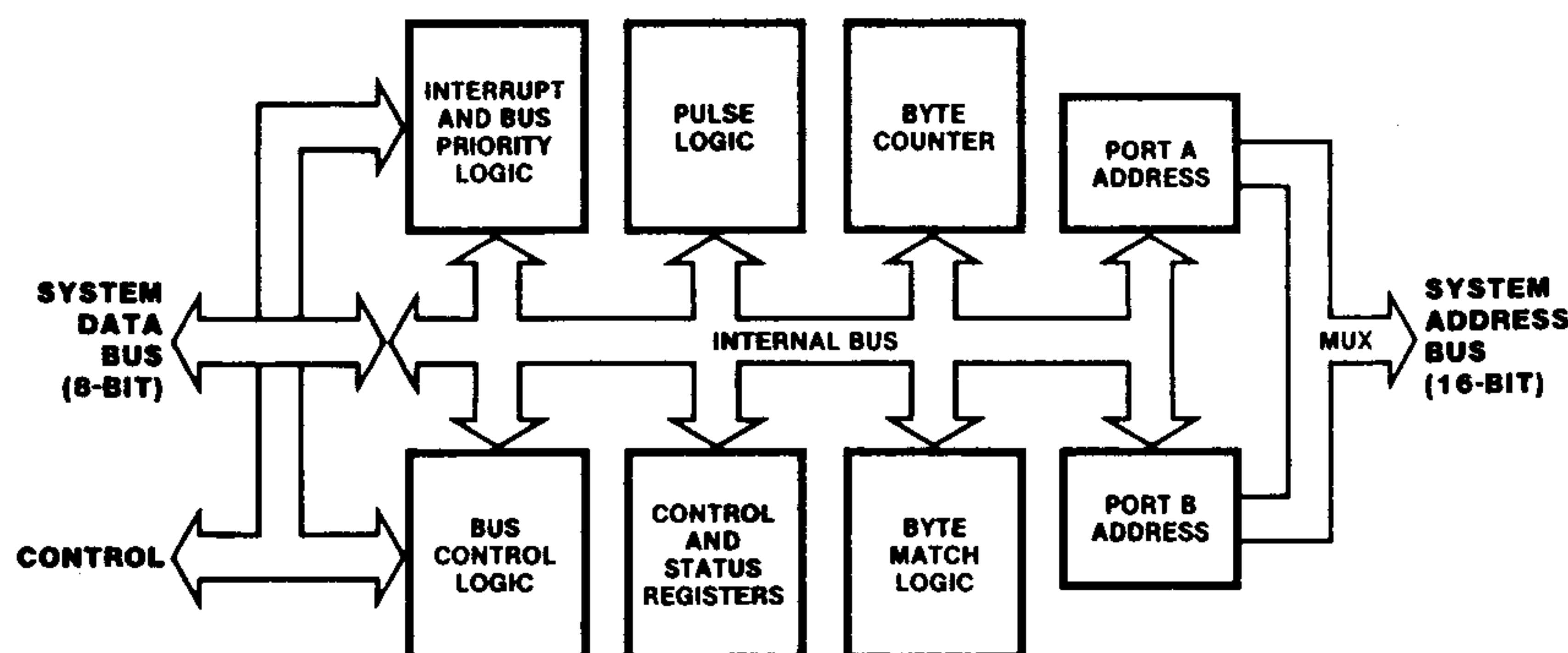
Figure 6. Block Diagram
