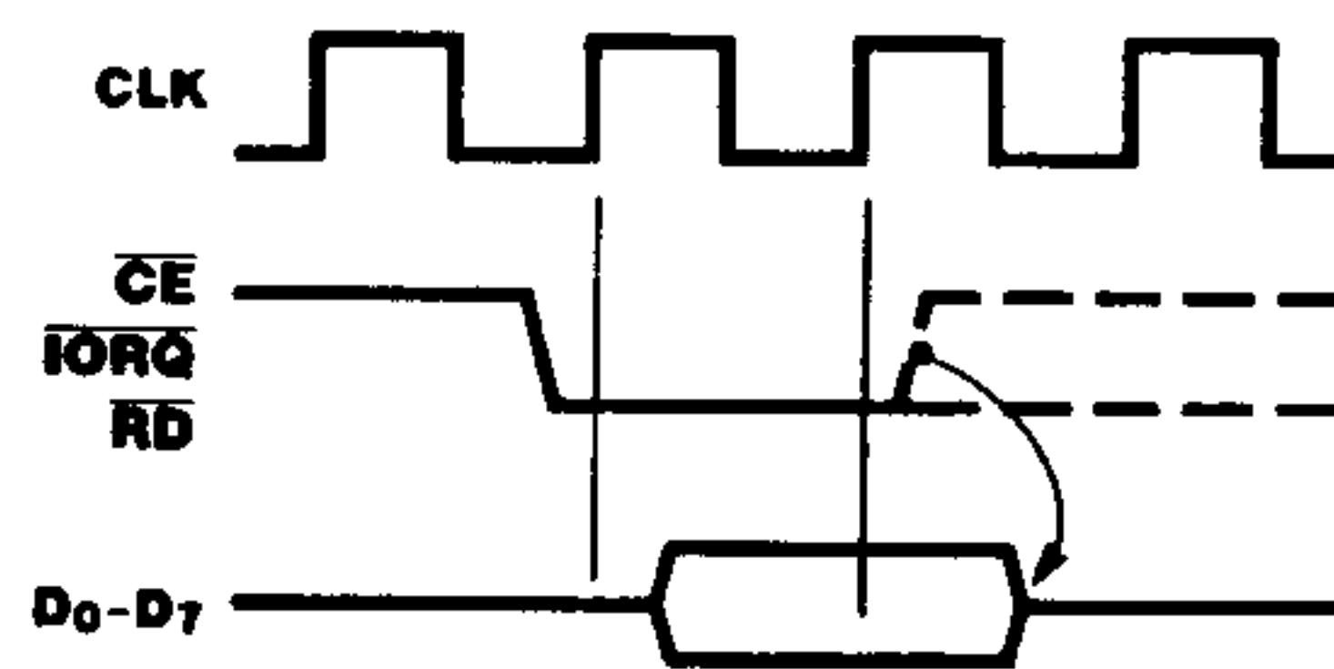
Figure 11. CPU-to-DMA Read Cycle
