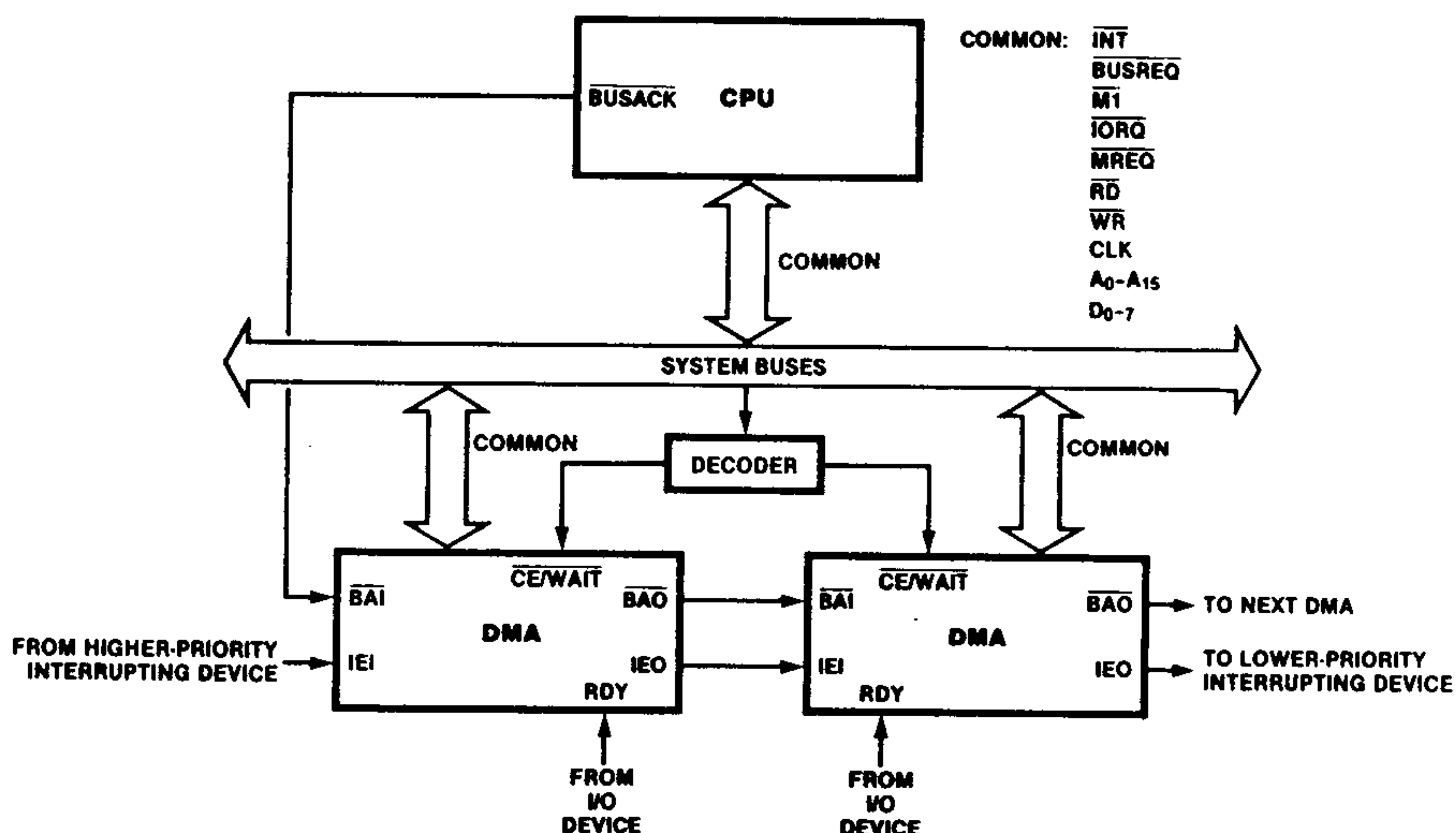
Figure 7. Multiple-DMA Interconnection to the Z80 CPU
