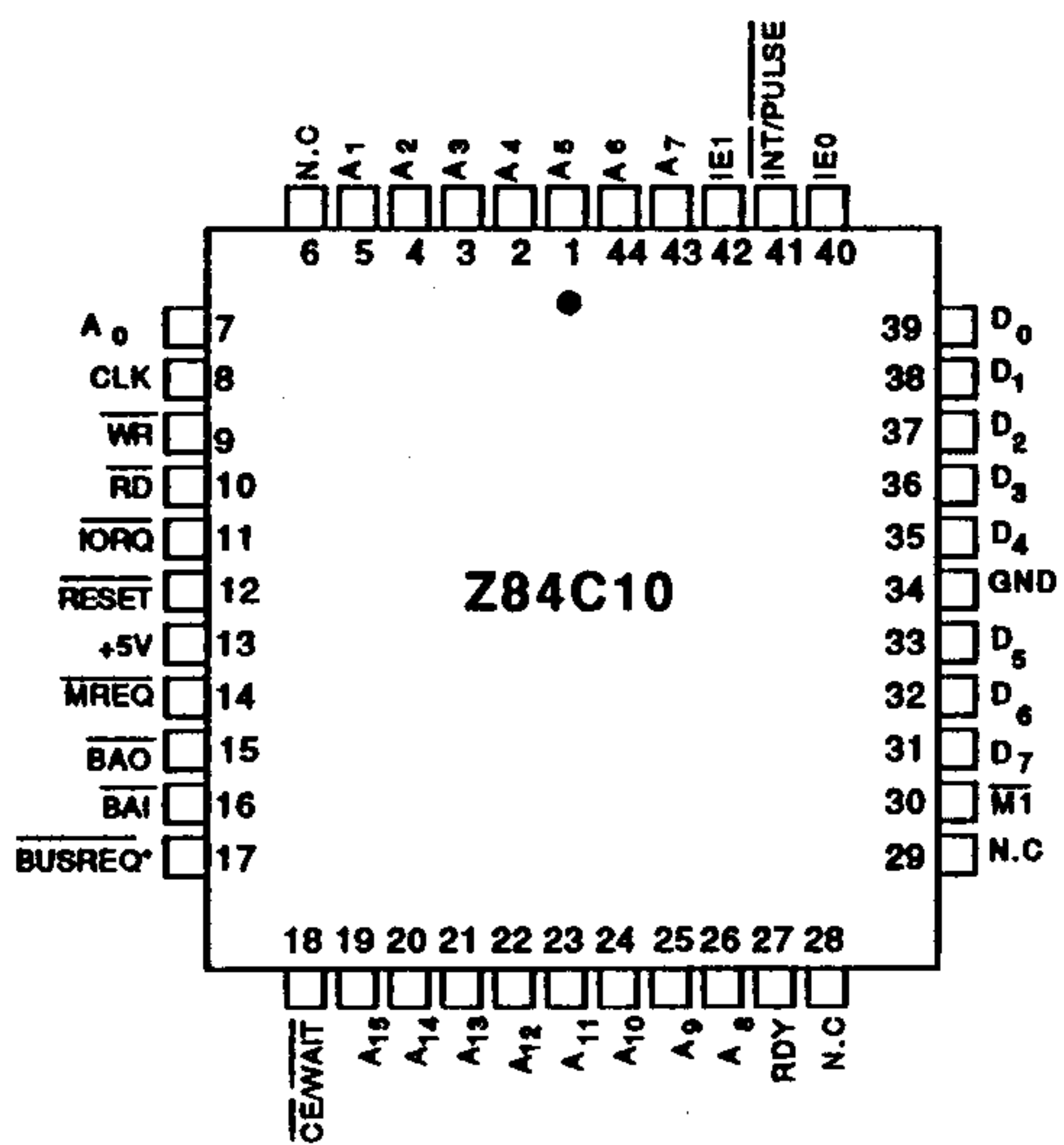
Figure 2c. Z84C10 CMOS Z80 DMA PLCC Pinout
