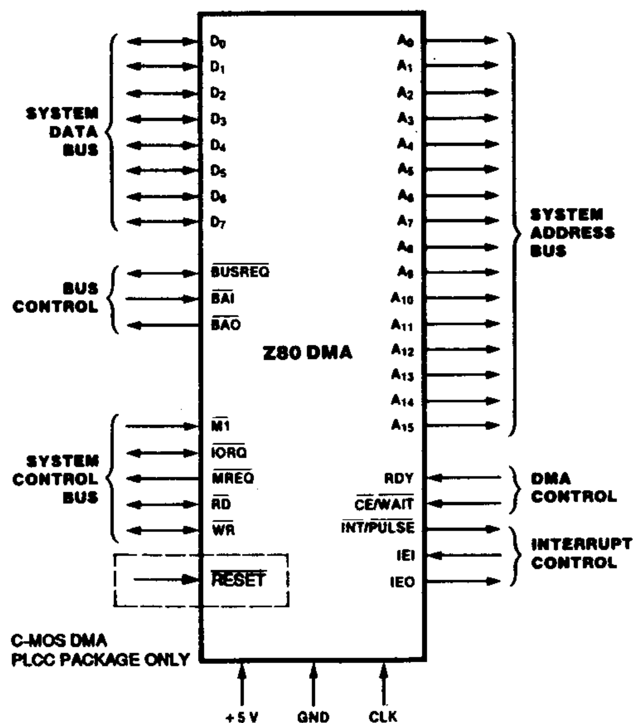
Figure 1. Pin Functions
