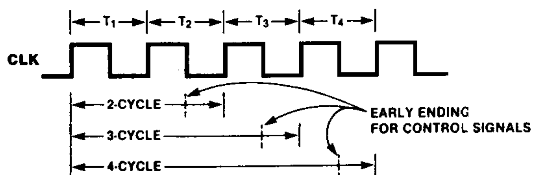
Figure 5. Variable Cycle Length
