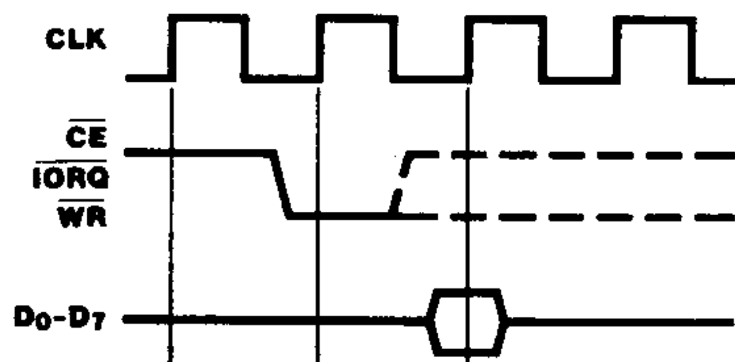
Figure 10. CPU-to-DMA Write Cycle
