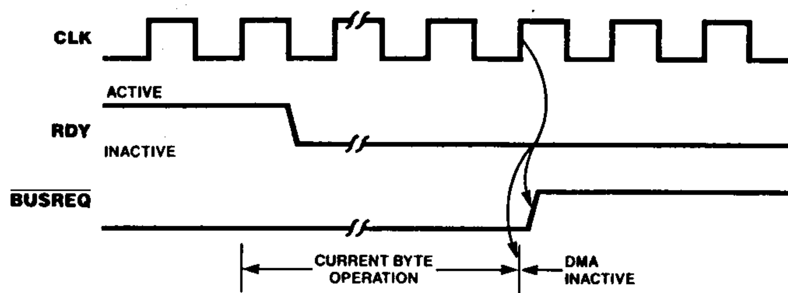
Figure 18. Bus Release When Not Ready (Burst Mode)
