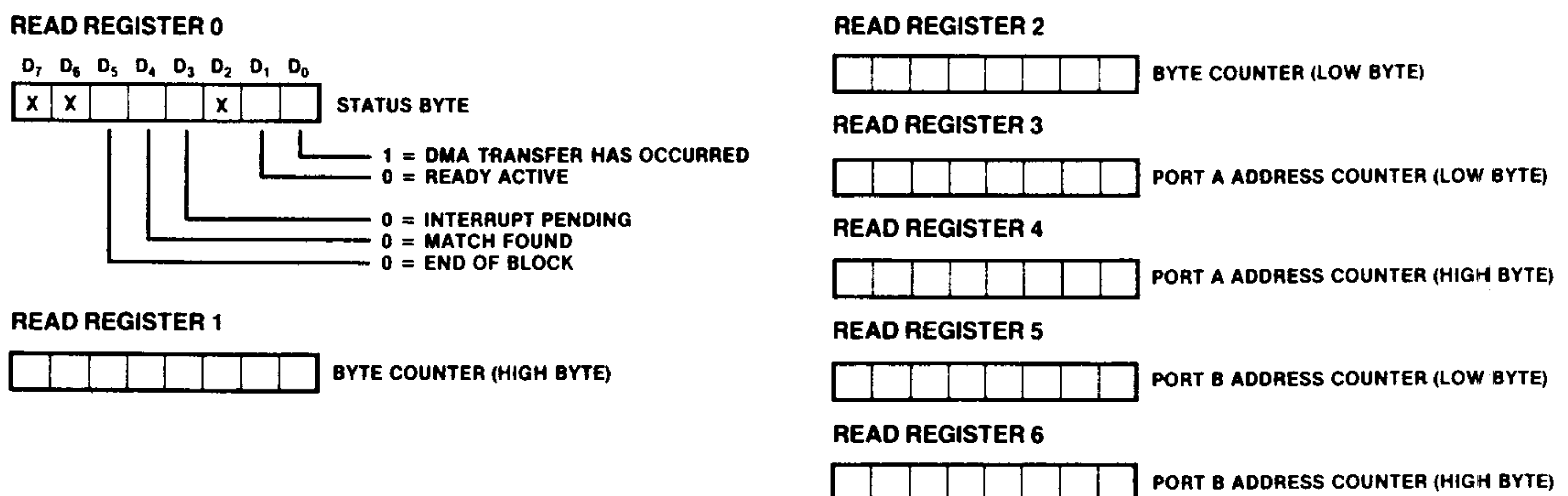
Figure 8a. Read Registers
