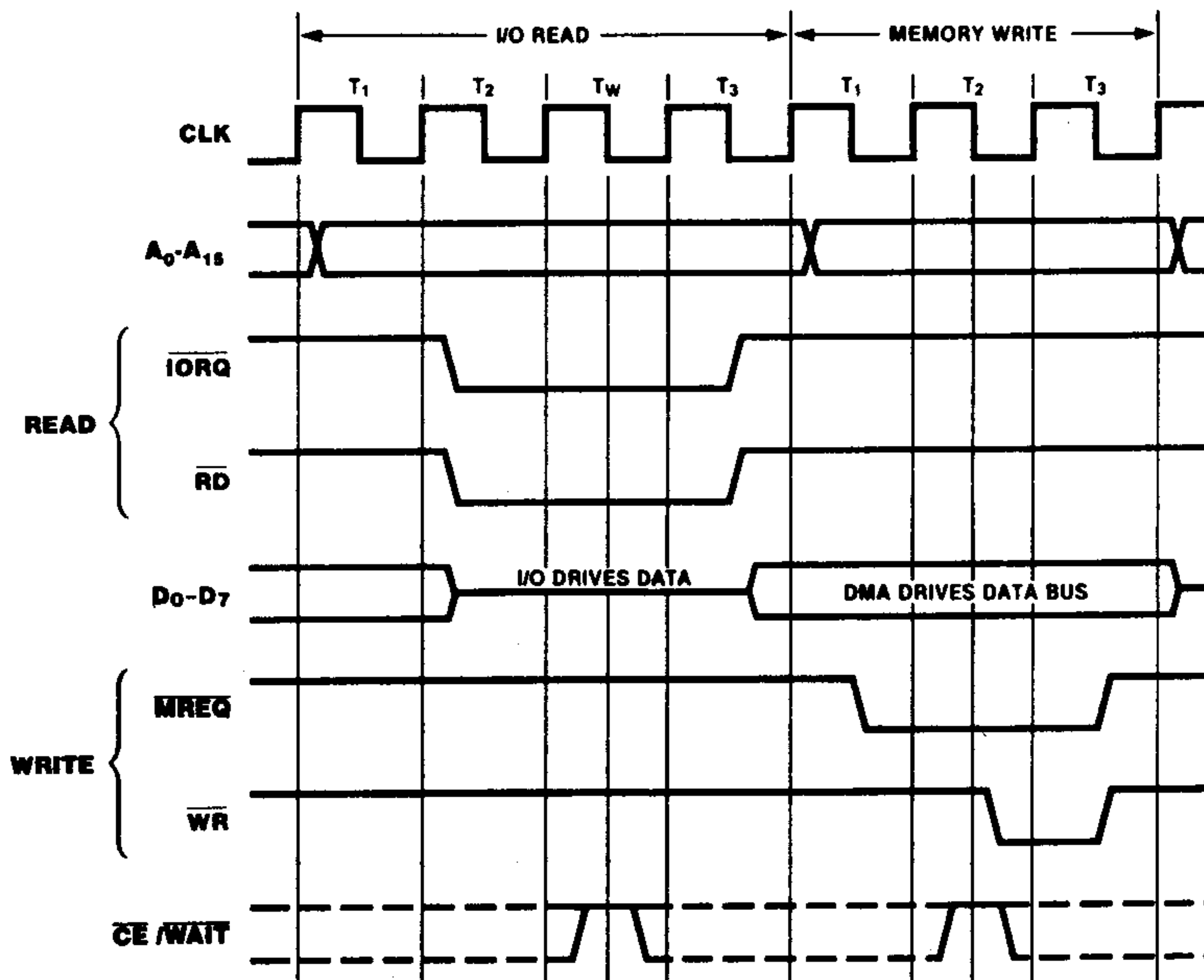
Figure 13. I/O-to-Memory Transfer
