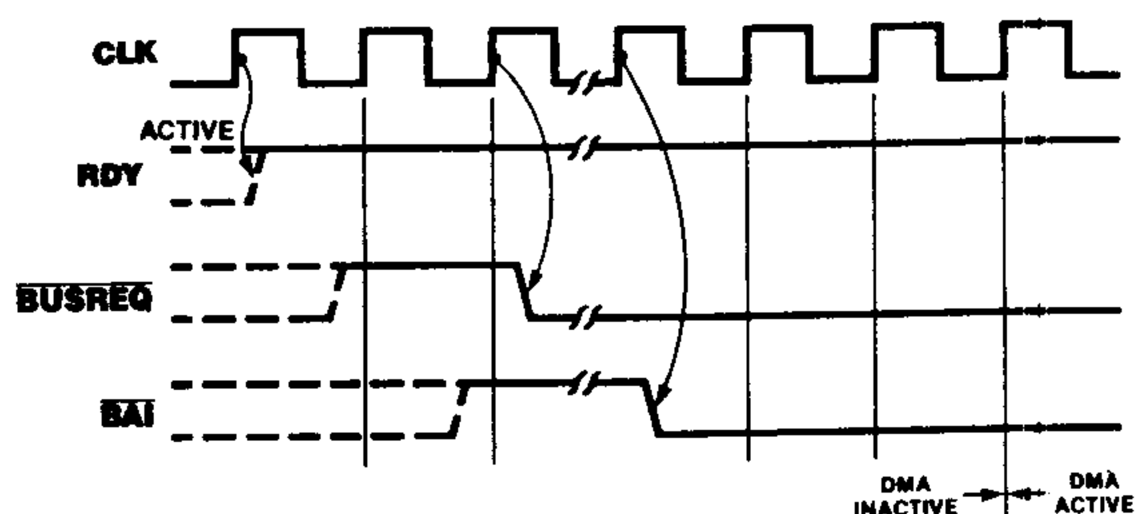
Figure 15. Bus Request and Acceptance
