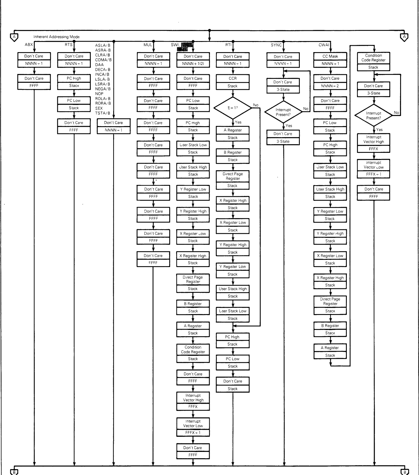
FIGURE 18 — CYCLE-BY-CYCLE PERFORMANCE (Sheet 2 of 5)
